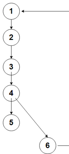
Gambar 2. Flowgraph login
